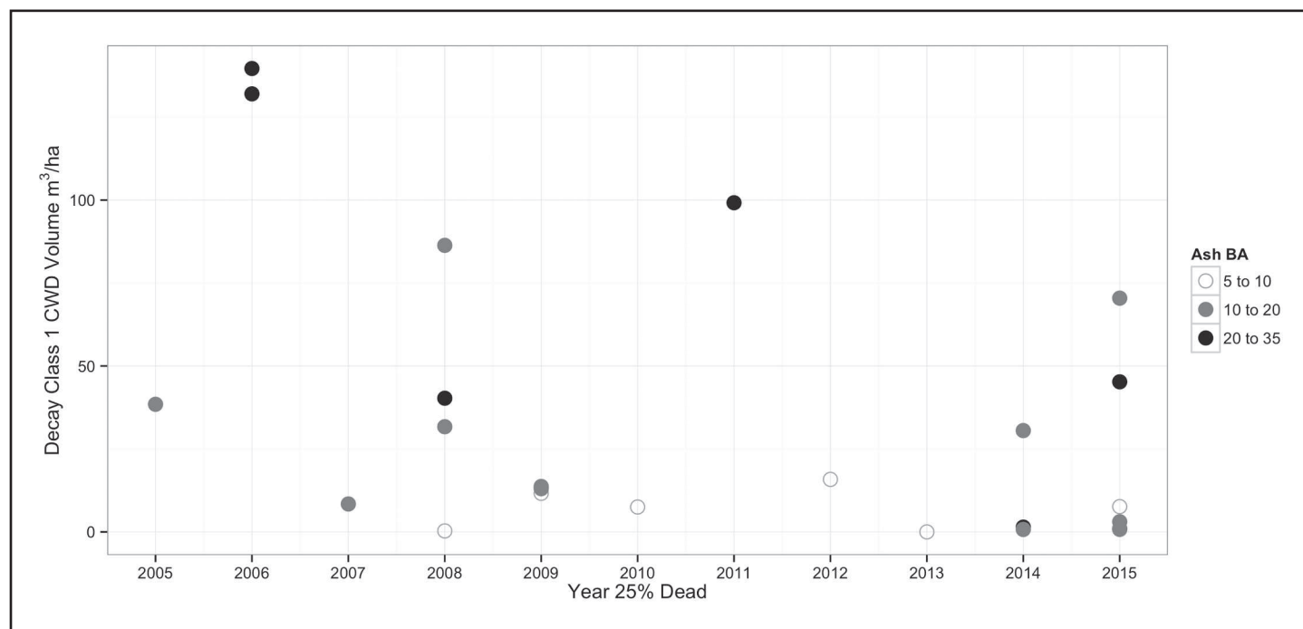
Figure 3. Scatterplot of average decay class 1 coarse woody debris (CWD) volume vs. year when ash mortality reached 25%, stratified by Fraxinus basal area (BA) in m²/ha, among study sites."
